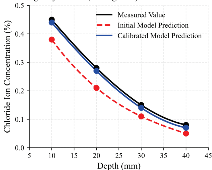
Figure 1 Chloride ion concentration distribution curve
